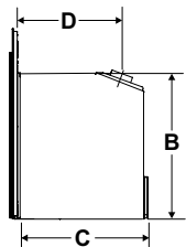
SIDE VIEW HRI6E, LRI6E, HRI4E, LRI4E, HRI3E, LRI3E, E33, L234
